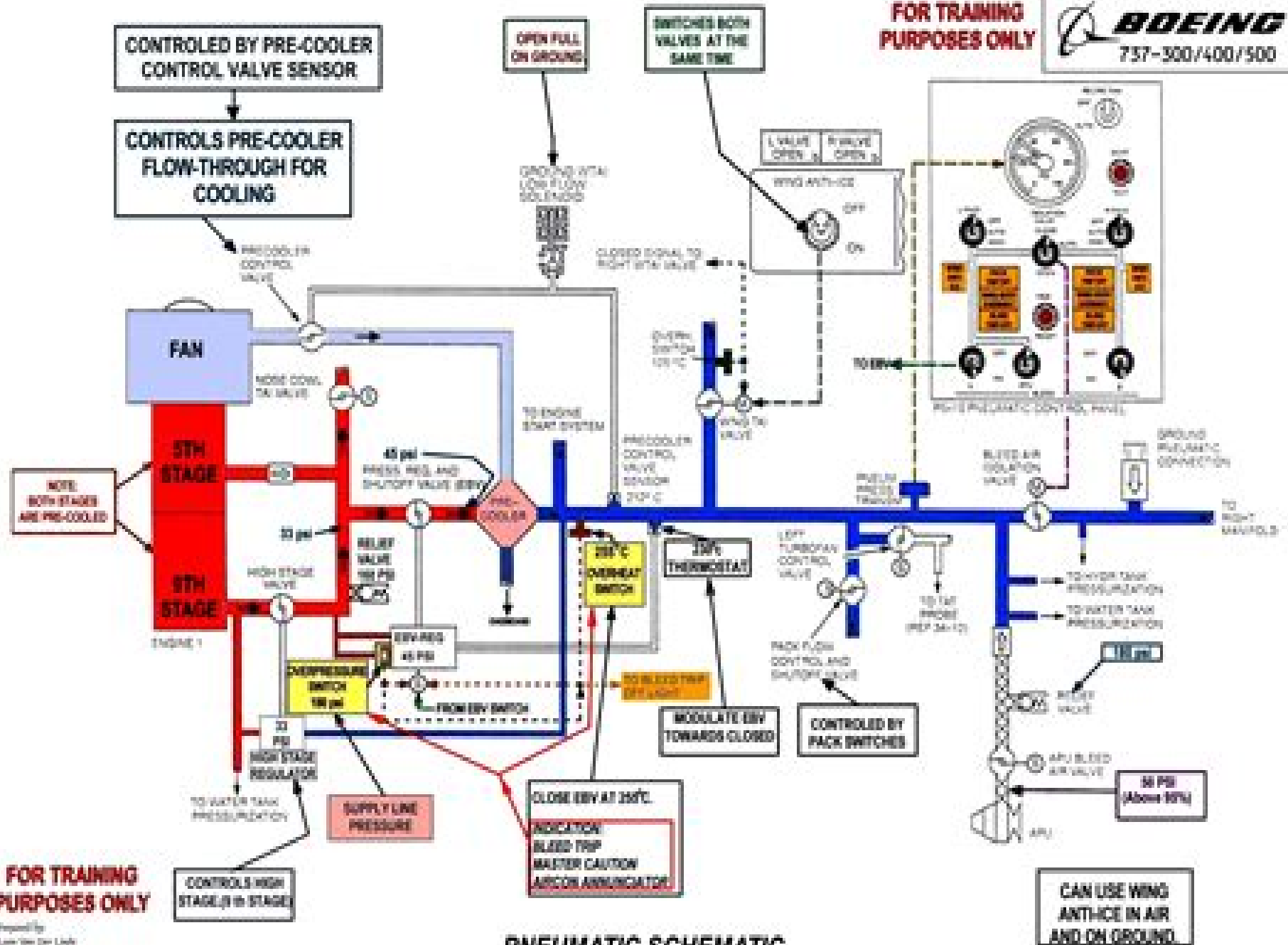
PNEUMATIC SCHEMATIC
