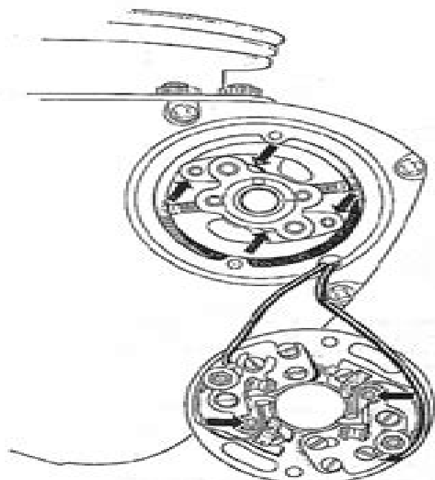
Fig. A10. Contact breaker mechanism lubrication points (MCA Contact breaker)
