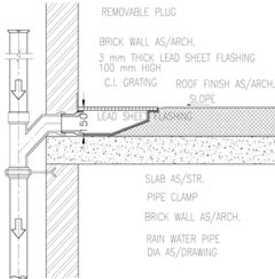
TYPICAL DETAIL OF ROOF DRAIN
