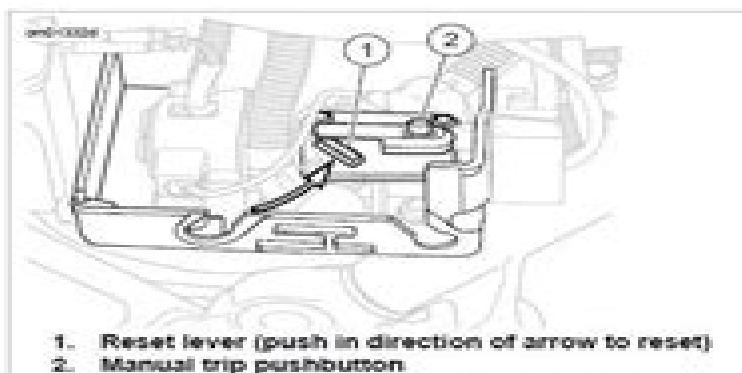
Figure 7-31. Reverse Motor Circuit Breaker
