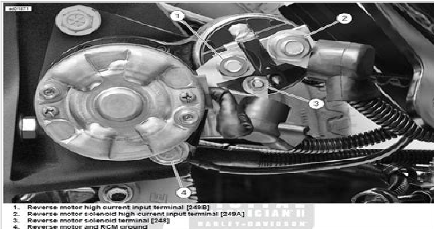
Figure 7-30. Reverse Motor and Solenoid Assembly
