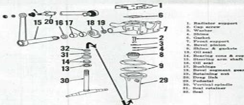
Fig. AC3—Models C and CA dual wheel tricycle version front support, pedestal, and front steering gear assembly.
