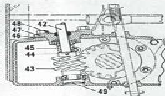
Fig. AC6—Models RC, WC, WD & WD45 single wheel, dual wheel, and adjustable axle type steering gear assembly.
