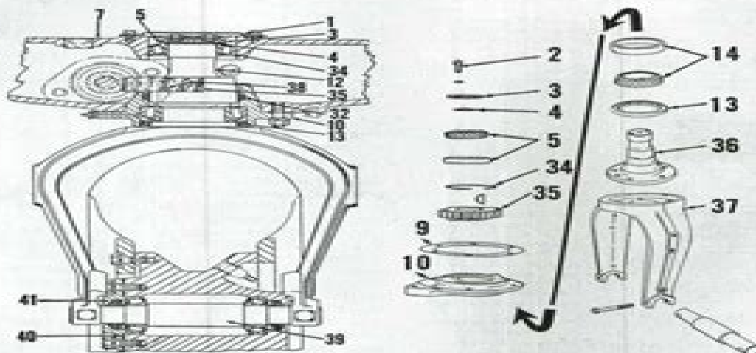
Fig. AC4—Models RC and WC single wheel tricycle version front support and main steering gear assembly. WD models prior to serial WD 25129 are similar.
