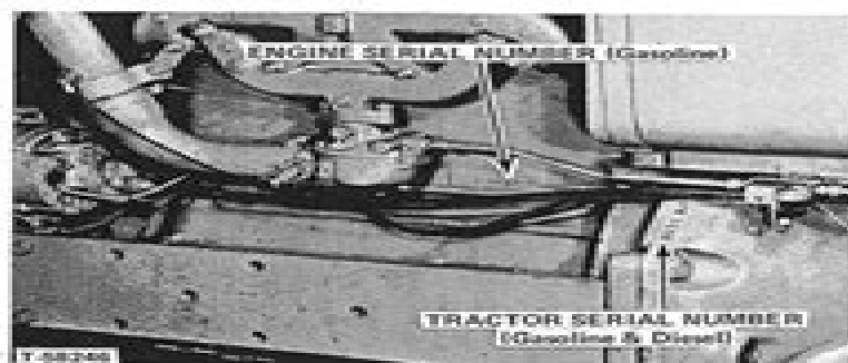
FIGURE 1 - Left Hand Side (Gasoline) (Shields Removed)
