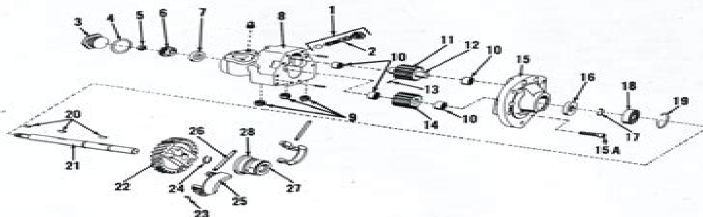
Fig. 15 — Exploded view of the D-17 non-diesel governor, distributor drive and power steering pump assembly used prior to tractor Serial No. D17-42001. Allen head screws (15A) retain the cover (15) to the body (8).
