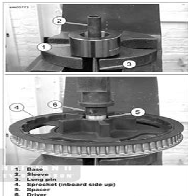
Figure 2-10. Remove Compensator Sprocket Bearing
