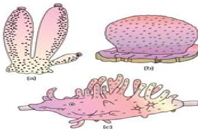
Figure 4.5 Examples of Porifera : (a) Sycon (b) Euspongia (c) Spongilia
