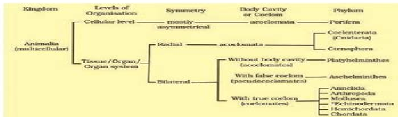
Figure 4.4 Broad classification of Kingdom Animalia based on common fundamental features
