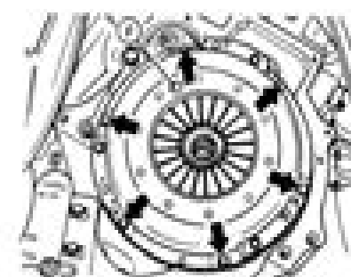
FIG 5.4 Removing clutch assembly from flywheel
