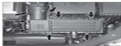
Air filter replacement for 2008 and later GTI models. 03 Maintenance
