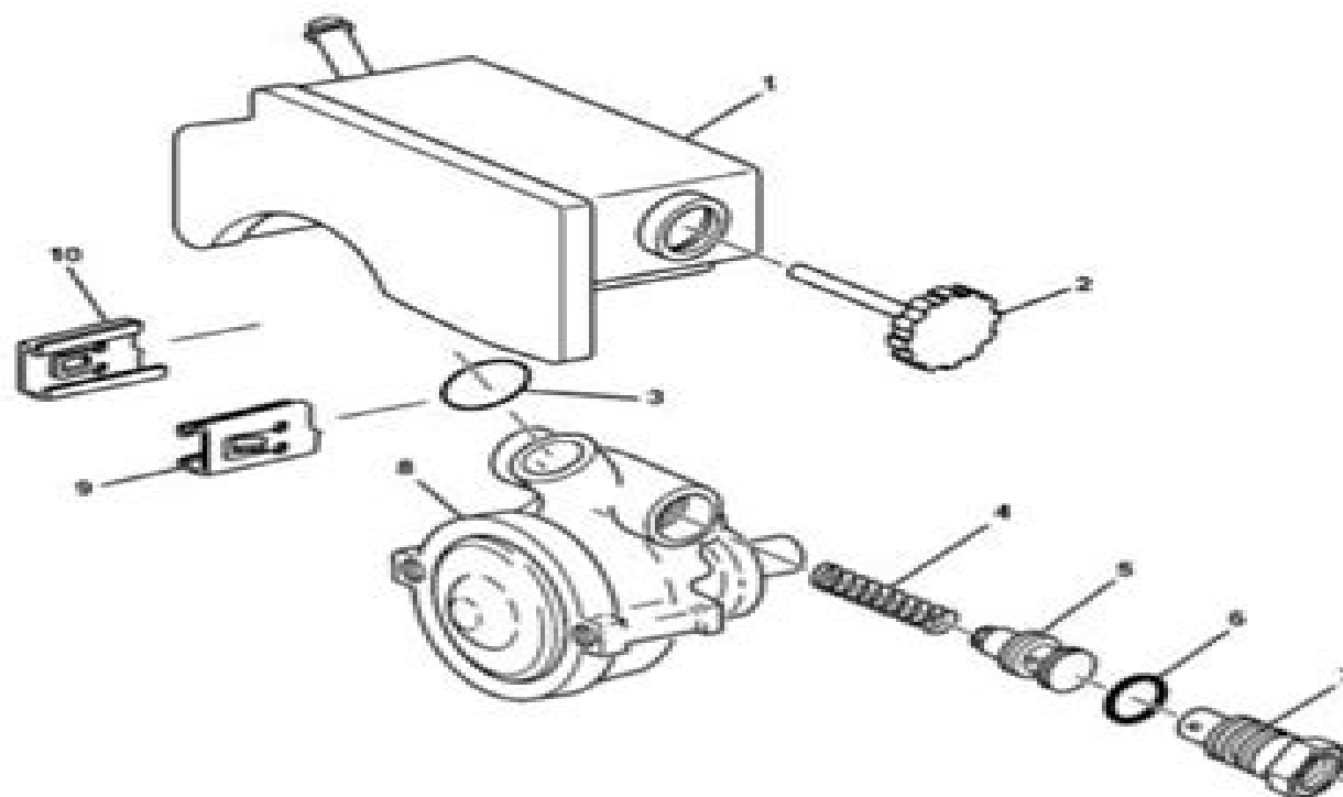
Fig. 2: Exploded View Of Power Steering Pump Components (CB Series) Courtesy of GENERAL MOTORS CORP.
