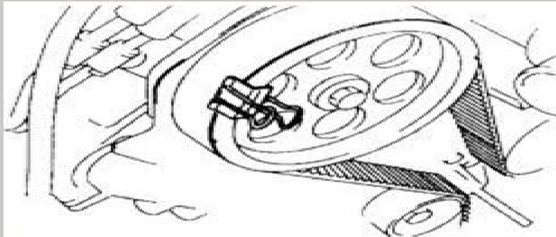
Fig. Fig. 14: Large paper clips are an excellent way to hold the belt in place during service. Timing belt tensioner pulley with pusher installed-3.2L engine
