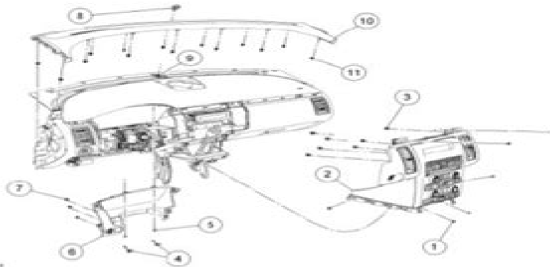
Fig. 9: Identifying Instrument Panel And Instrument Cluster Finish Panels Courtesy of FORD MOTOR CO.
