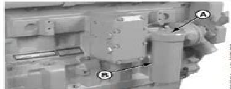
Removing Filter and Valve Housing
