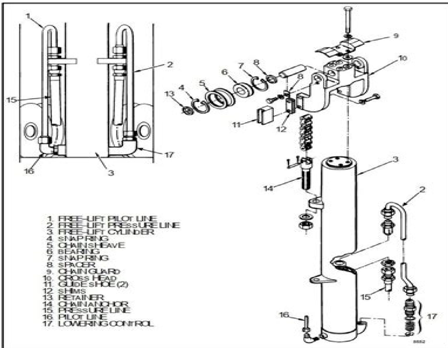
FIGURE 5. MAST WITH A FREE-LIFT CYLINDER (1 of 2)
