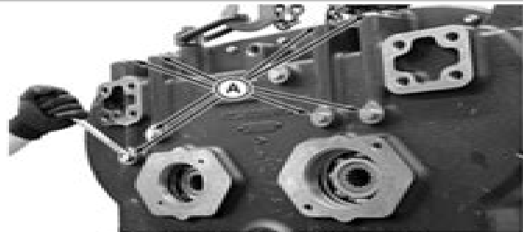
Pump Drive Housing Oil Passage Plugs
