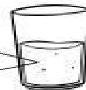
liquid water
