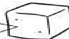
ice
