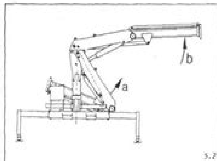
5.2 Raise boom (a) out of set-down position until jib (b) can be folded out safely.
