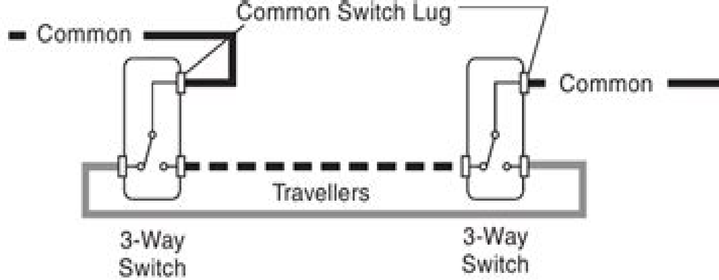
Existing Wiring Diagram
