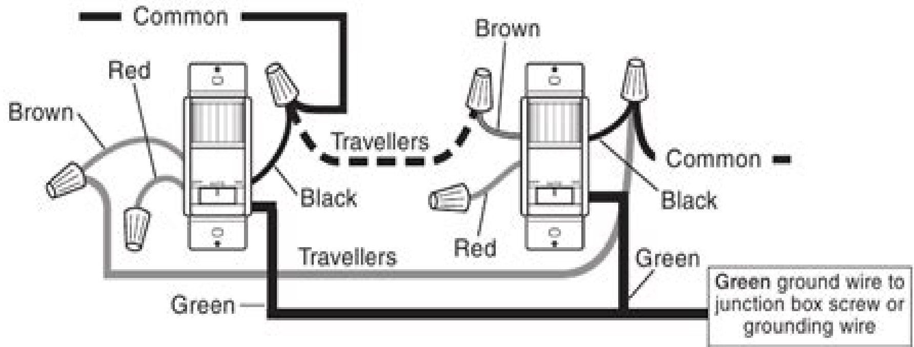
Existing Wiring Diagram
