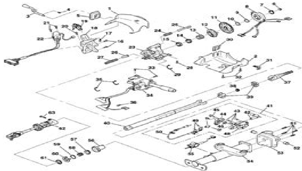
Fig. 2: Tilt Steering Column Disassembled View, Column Shift Courtesy of GENERAL MOTORS CORP.
