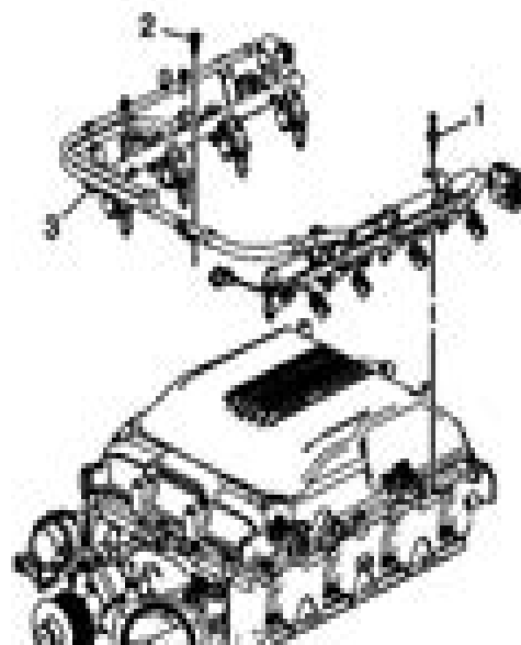
Fig. 26. Identifying Fuel Rail Components Courtesy of GENERAL MOTORS COMPANY
