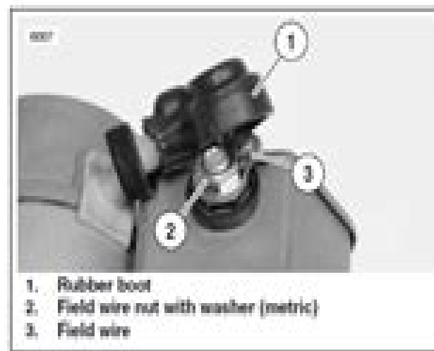
Figure 5-14. Field Wire
