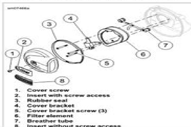
Figure 1-5. Air Cleaner Assembly
