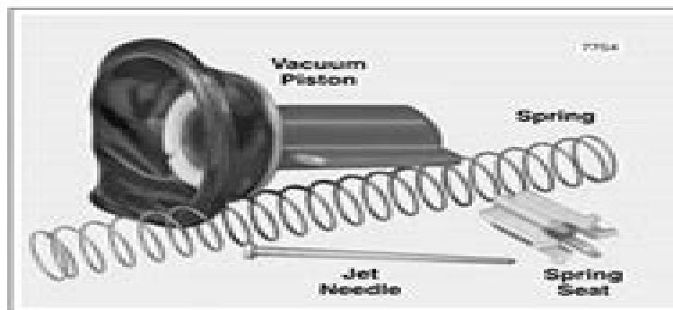
Figure 4-7. Carburetor-Top End
