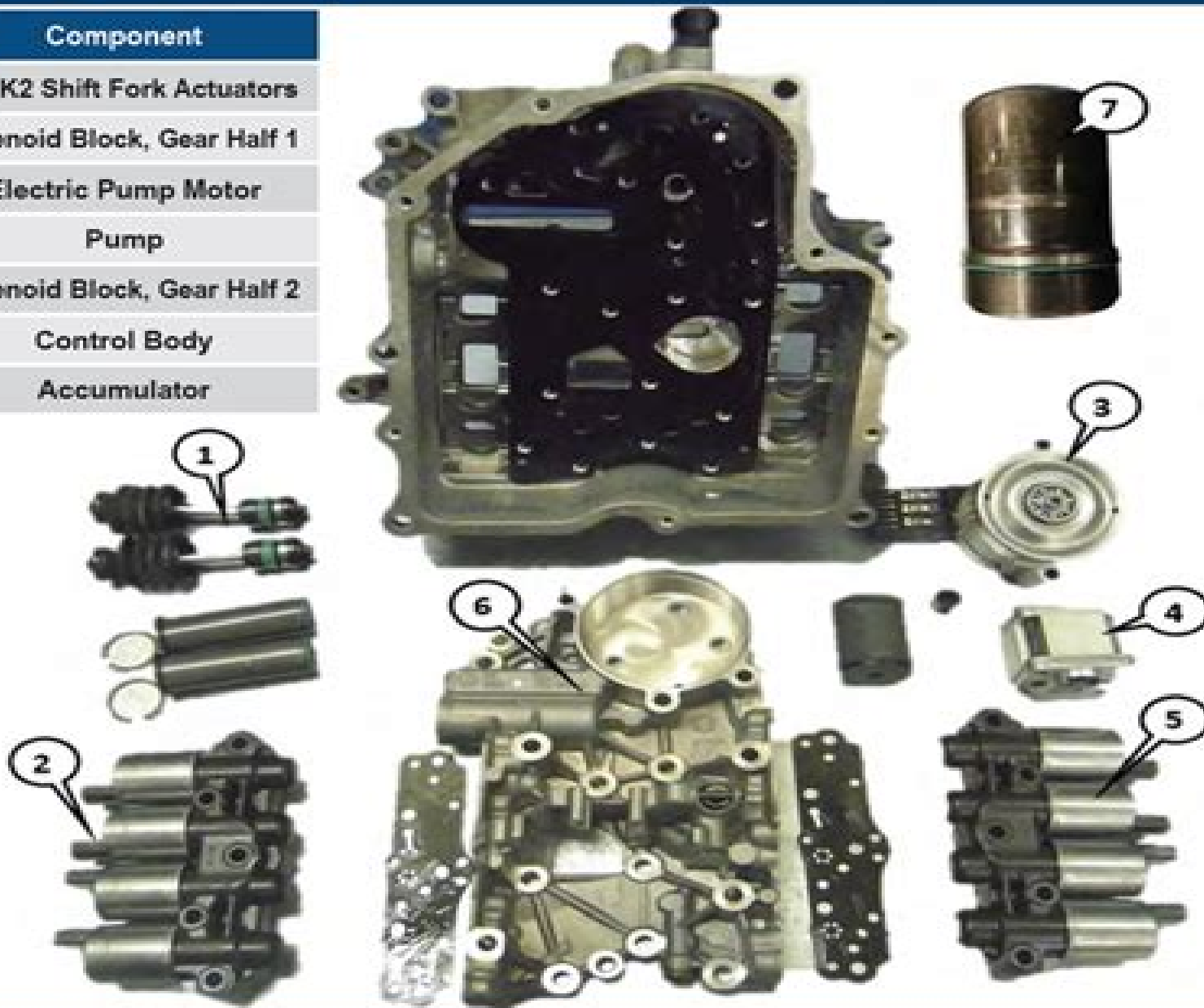
Figure 2: Most of the components inside the Mechatronic assembly are serviceable with parts available through aftermarket resources. Note, the oil pump is a high pressure pump capable of producing up to 1,015 psi (70 bar) of pressure in fail safe mode!
