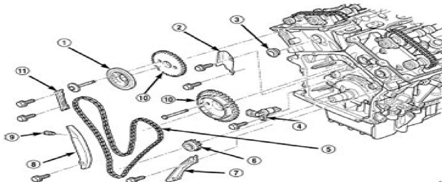
Fig. 118 TIMING DRIVE SYSTEM - PRIMARY
