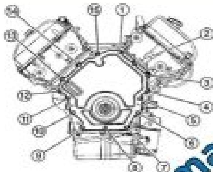
Fig. 12: Installing Timing Chain Cover to Camshaft of GENERAL MOTORS V-6
