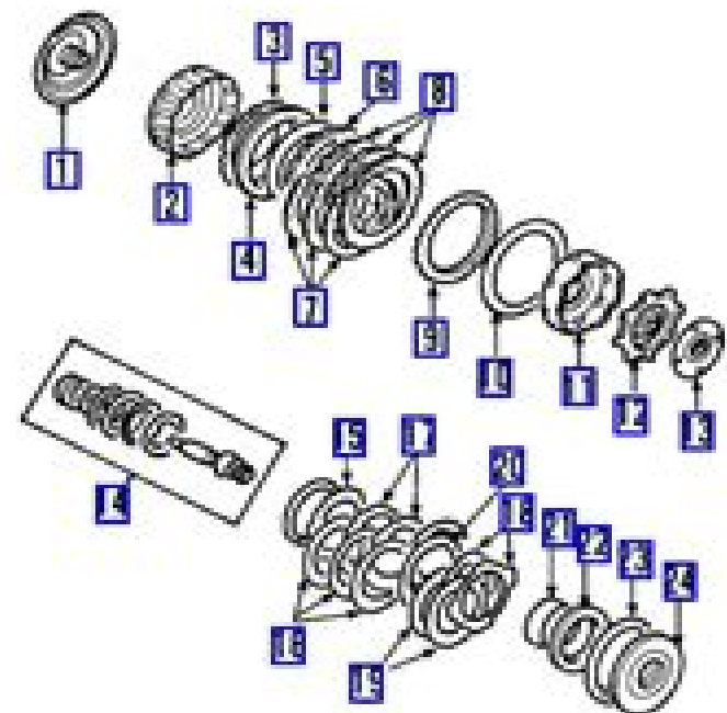
CLUTCHES & PLANETARY GEARS
