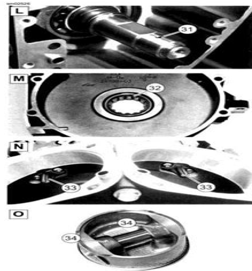
Figure 3-3. Engine Oil Flow-Bottom End
