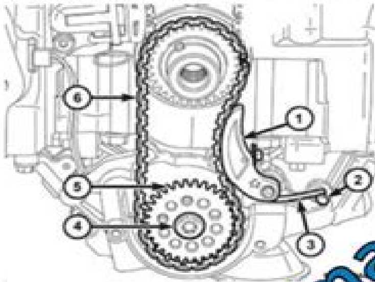
Fig 16: Oil Pump Chain Tensioner Spring, Cover Pin, Oil Pump Chain Tensioner, Oil Pump Sprocket, Retaining Bolt & Oil Pump Chain
