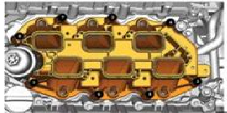
Fig 2: Lower Intake Manifold Bolt Removal & Tightening Sequence
