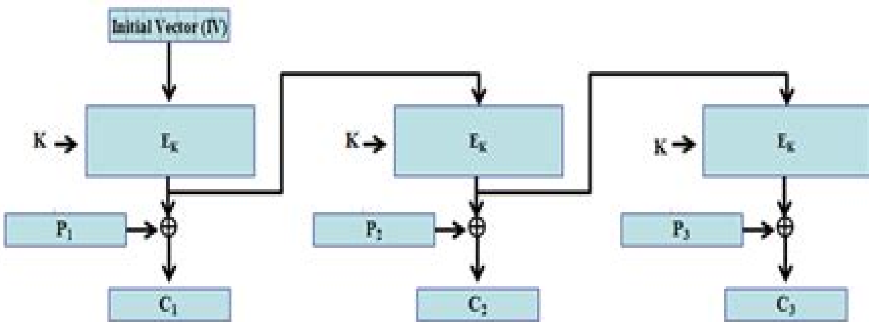
a) Output feedback (OFB) encryption mode
