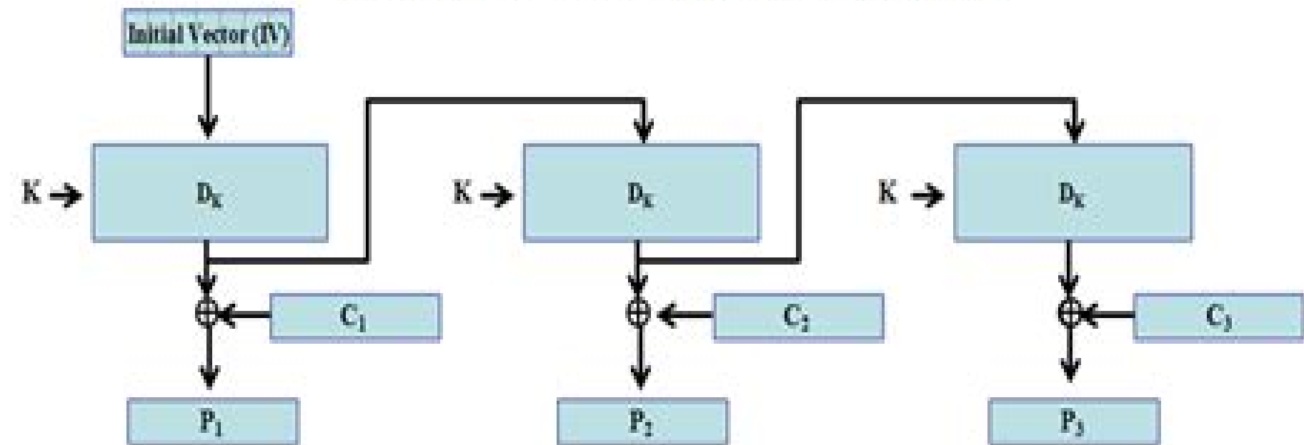
a) Output feedback (OFB) decryption mode
