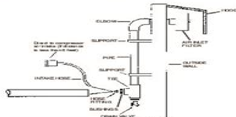
Typical Remote Air Inlet Piping.
