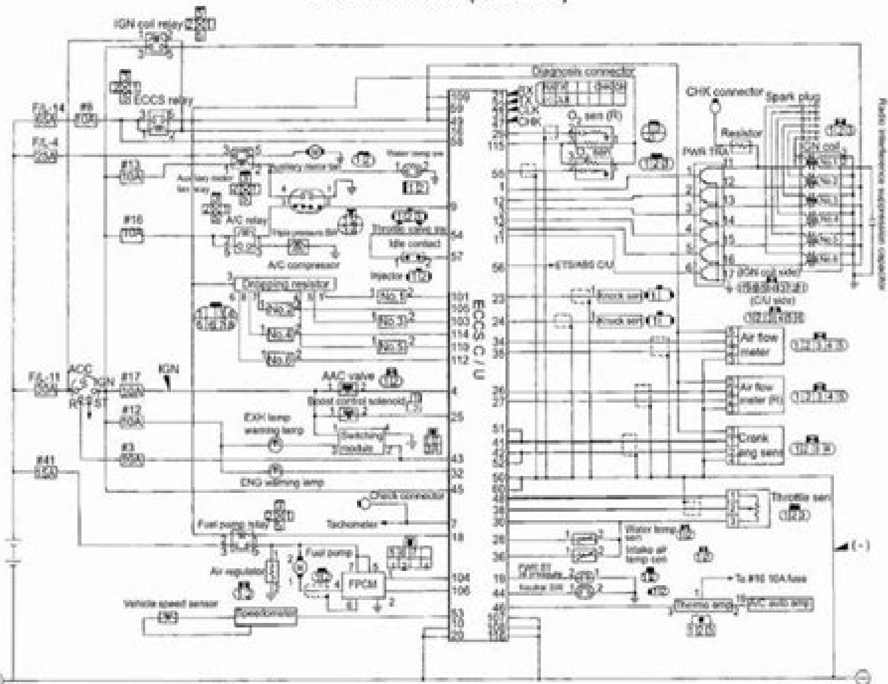
CIRCUIT DIAGRAM (RB26DET)
