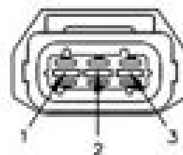
RAIL FUEL PRESSURE SENSOR CONNECTOR MATING FACE
