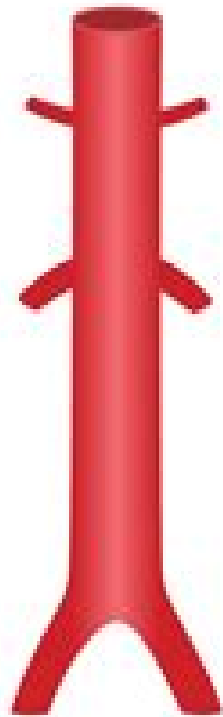
Healthy abdominal aorta
