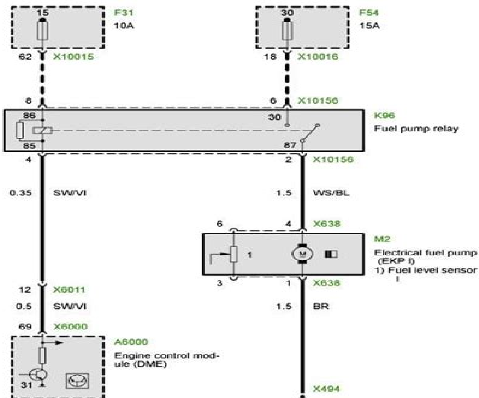
E39 Fuel pump
