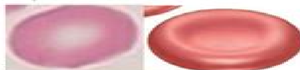
Biconcave shape
