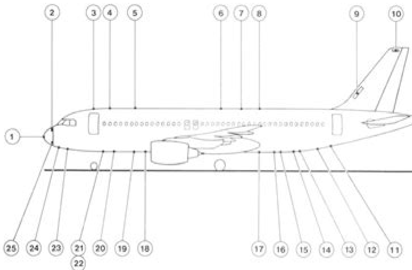
Fig. 23-1 Antennas locations www.british-aviation.com
