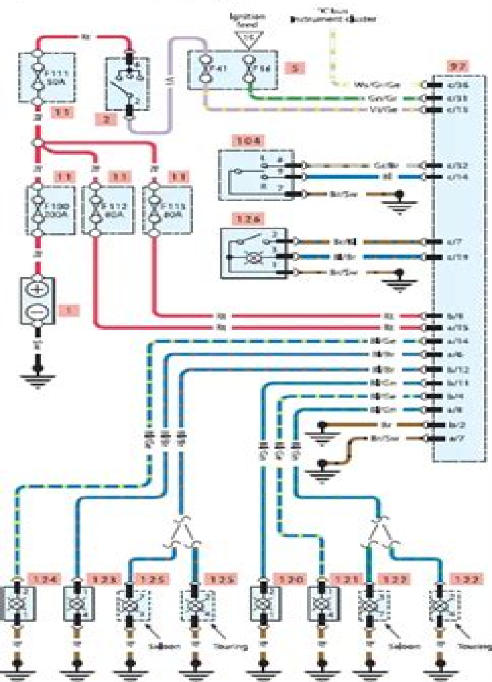
Typical direction indicators & hazard warning lights
