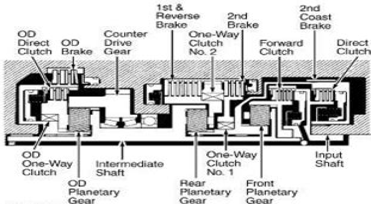
Fig. 4: Identifying Transaxle Component Locations Courtesy of TOYOTA MOTOR SALES, U.S.A., INC.
