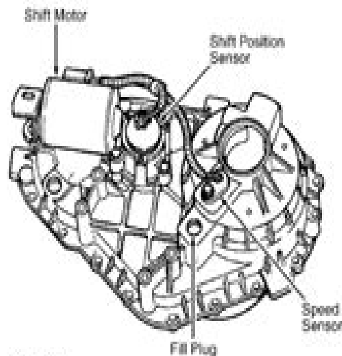
GMW4405 Fig. 1: Identifying Model 4405 Transfer Case Courtesy of Ford Motor Co.
