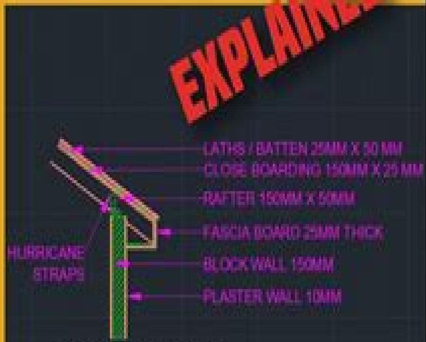
CLOSED EAVE DETAIL
