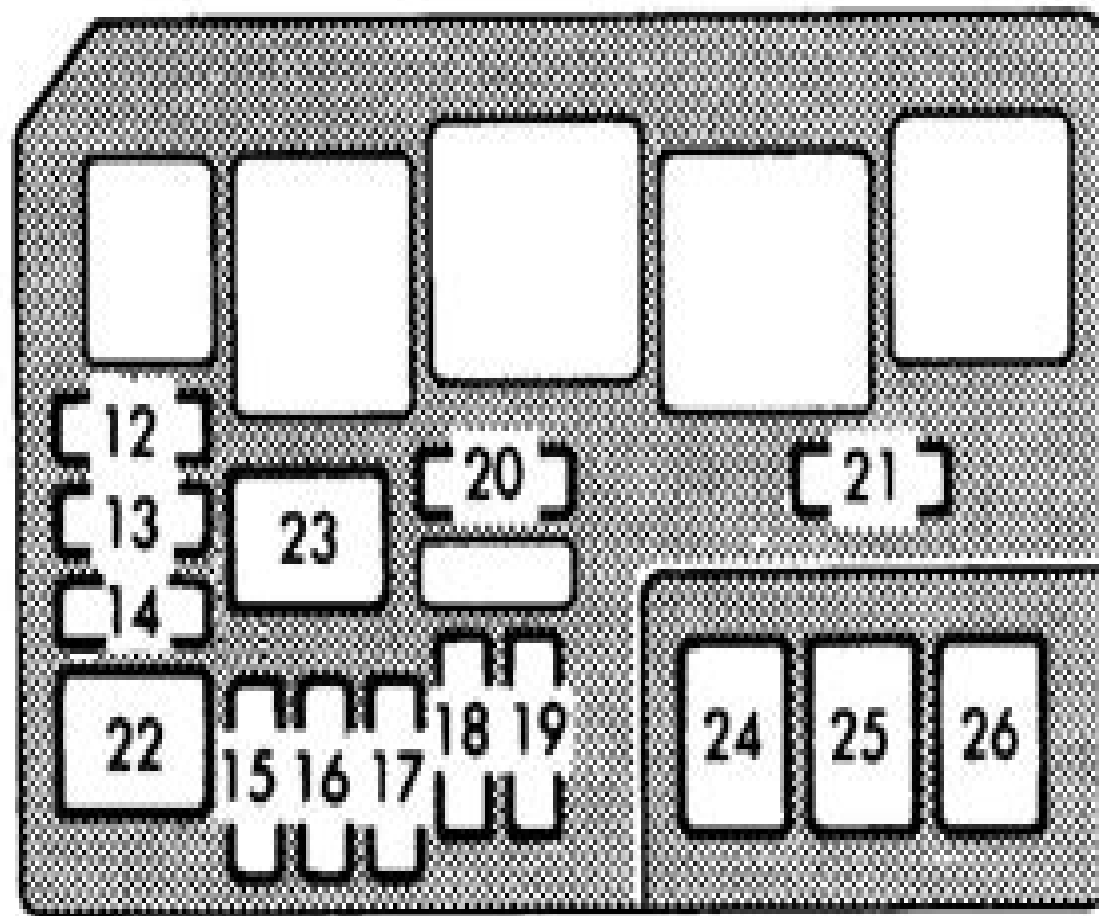
ENGINE COMPARTMENT
