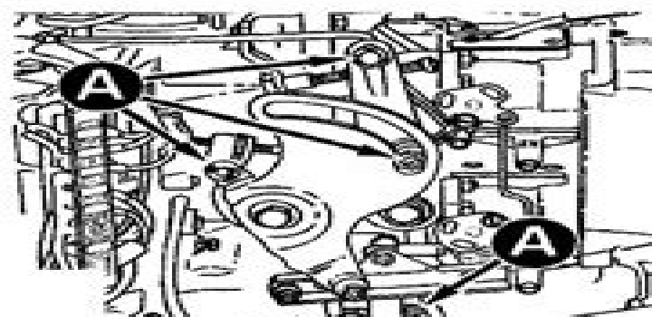
Fig. 20 Carburetor, throttle and shift linkage lubrication points-65 Jet-115 Hp (1632cc) V4 motors
