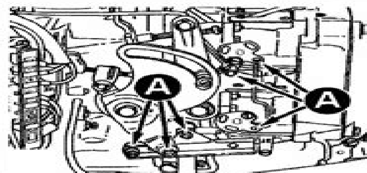
Fig. 20 Carburetor, throttle and shift linkage lubrication points-65 Jet-115 Hp (1632cc) V4 motors
