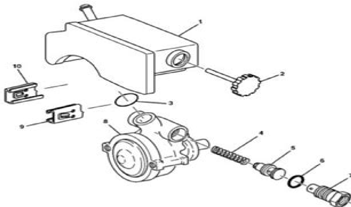
Fig. 2: Exploded View Of Power Steering Pump Components (CB Series) Courtesy of GENERAL MOTORS CORP.
