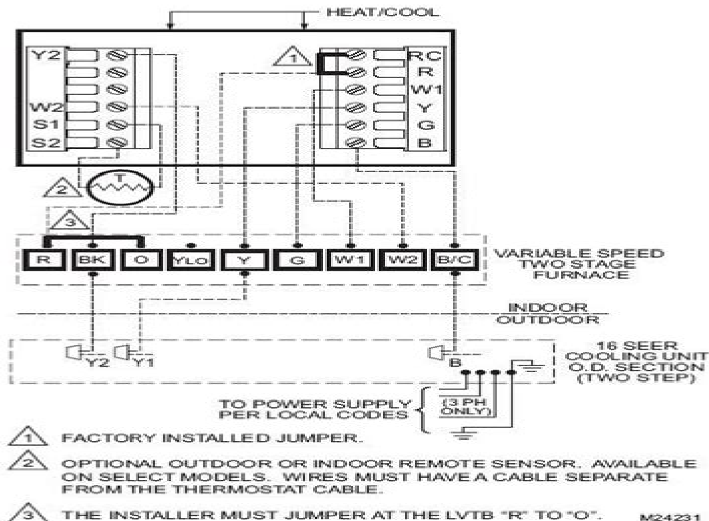
Fig. 8. Typical hookup of two-stage indoor and two-step scroll cooling unit in a single transformer system (2H/2C or 2H/1C or 1H/2C).
