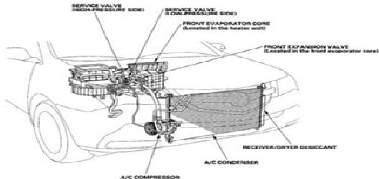
Fig. 1: Identifying Climate Control Component Location (1 Of 3) Courtesy of AMERICAN HONDA MOTOR CO., INC.
