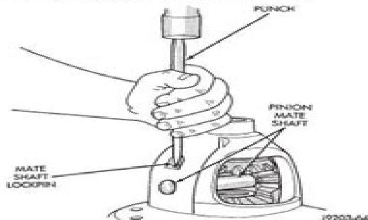
Fig. 40 Mate Shaft Pin Installation
