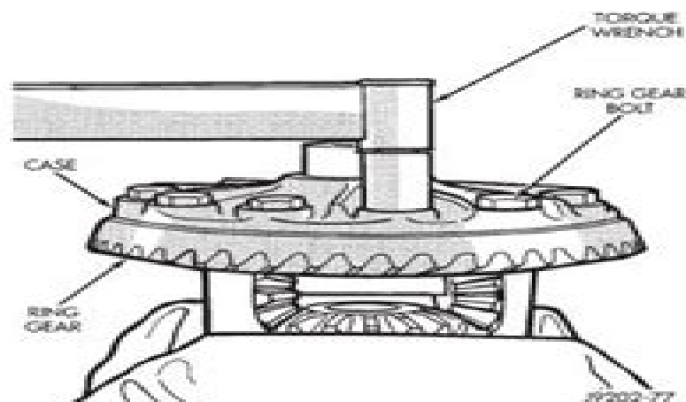
Fig. 41 Ring Gear Bolt Installation
