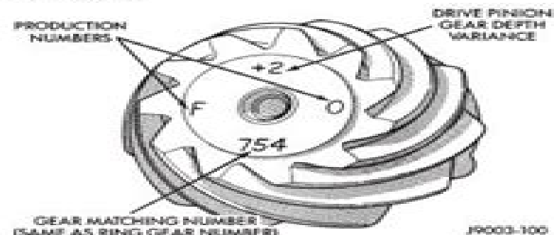
Fig. 42 Pinion Gear ID Numbers
