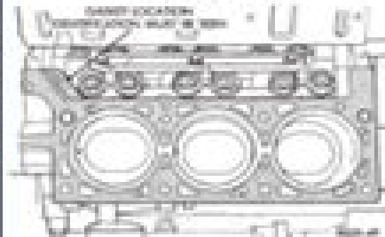
Fig. 32 Head Gasket Installation
